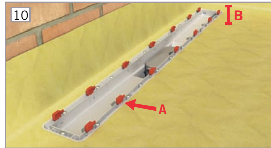
10 Choose the pin A and its position according to the tile thickness B and the selected adhesive.
