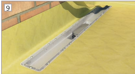
9 Cut and remove the unused part of the water tightening fabric.
